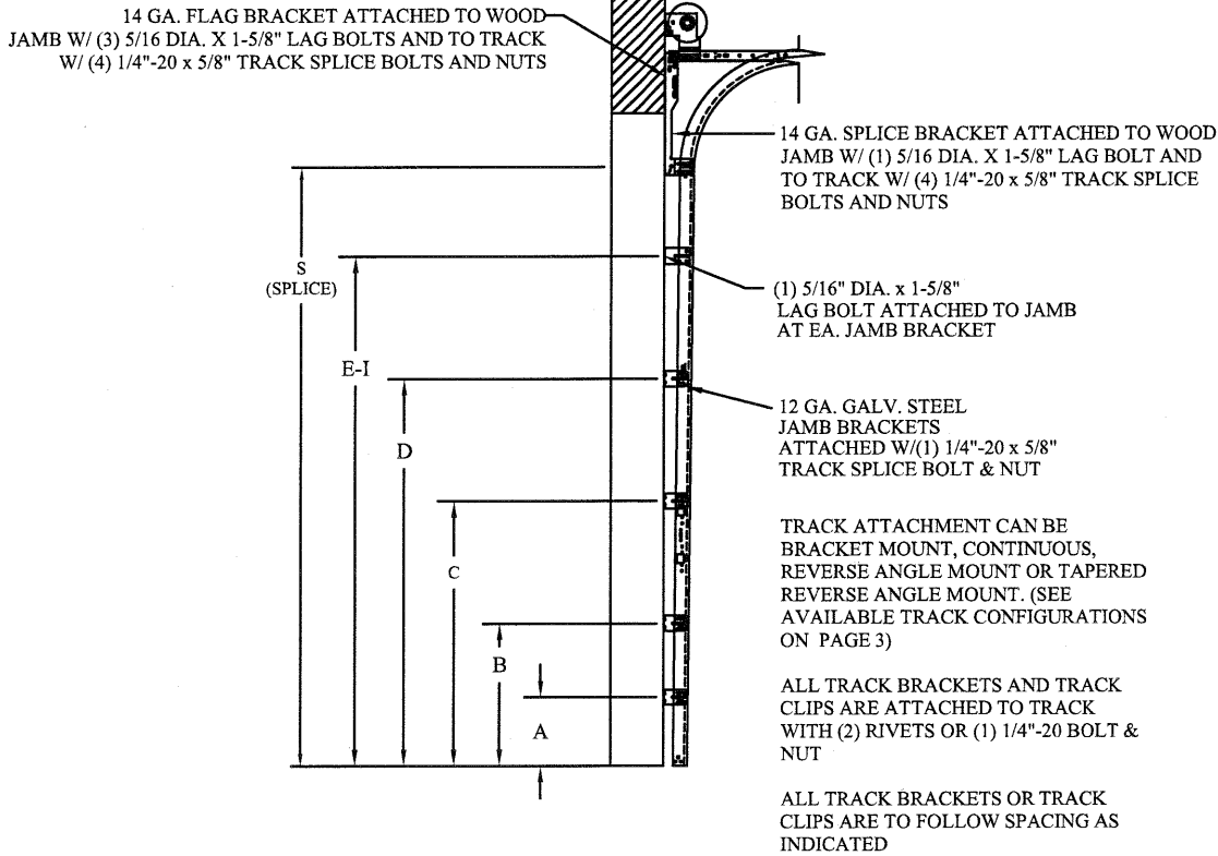
TRACK CONFIGURATION FOR 8' TALL DOORS N.T.S. SEE TABLE 1 FOR TRACK ATTACHMENT SPACING
